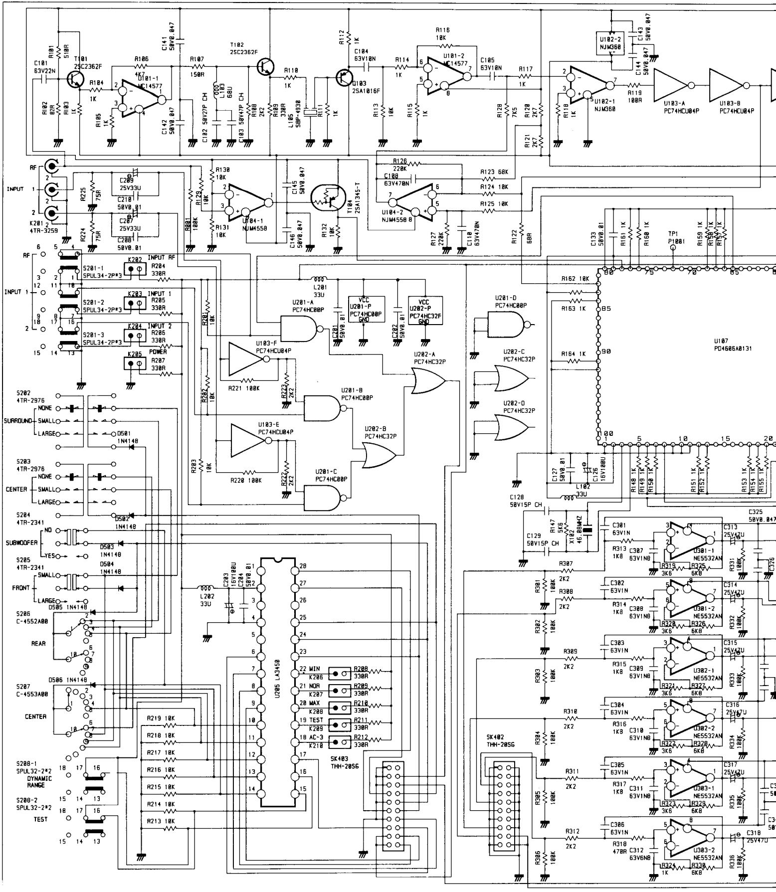
SCHEMATIC DIAGRAM MODEL NO. RDA-980
