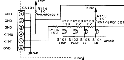
TO MOTHER ASSY CN104 (SCH-4)
