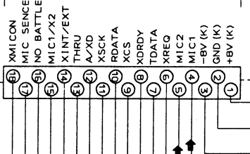
TO KRAB ASSY CN102 (SCH-6)
