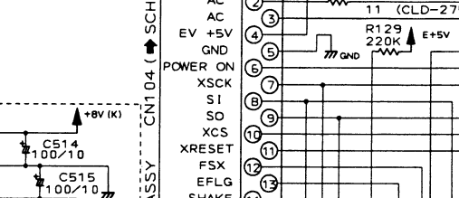
TO MOTHER ASSY CN104 (SCH-4)
