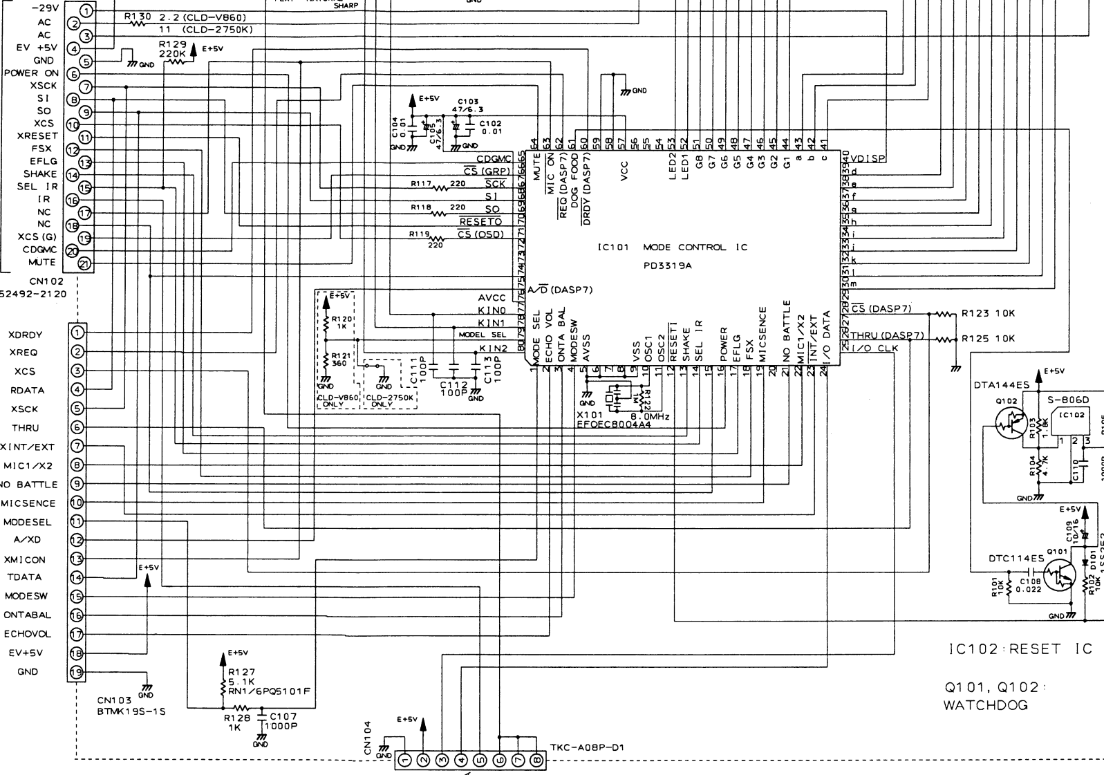
TO MOTHER ASSY CN104 (SCH-4)
