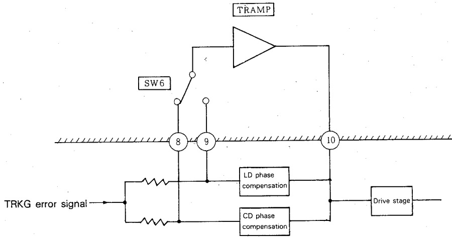
Fig. 16-3-9 CD/LD switching
