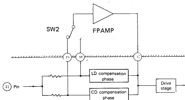
Fig. 16-3-3 CD/LD switching
