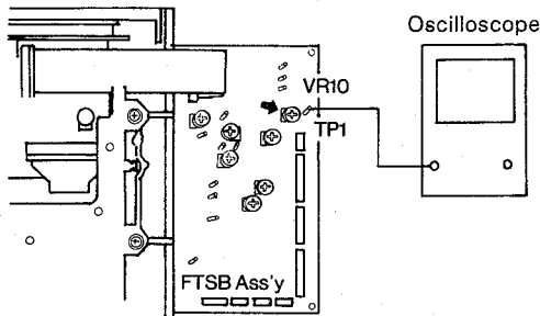
2. Connect FTSB ass'y TP1 to an oscilloscope
